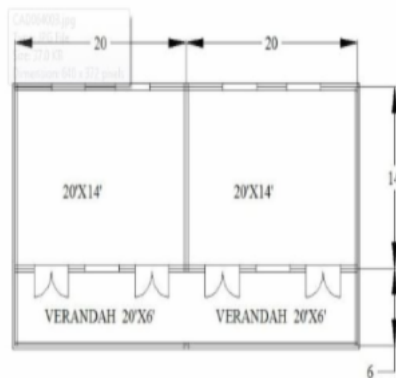
Cad View
