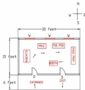
Cad View
