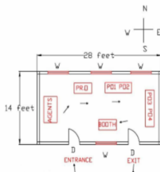
Cad View
