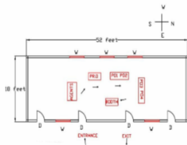
Cad View
