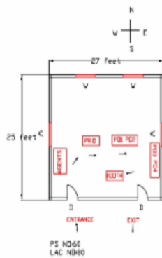
Cad View
