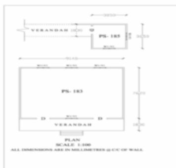
Cad View
