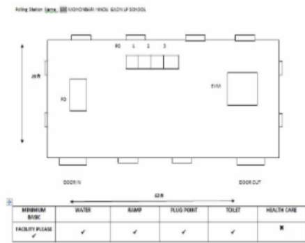
Cad View
