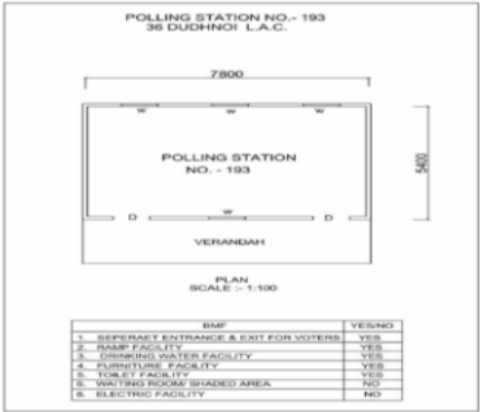
Cad View
