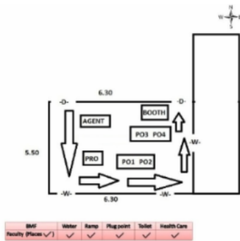
Cad View
