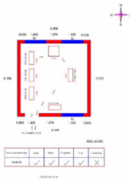
Cad View
