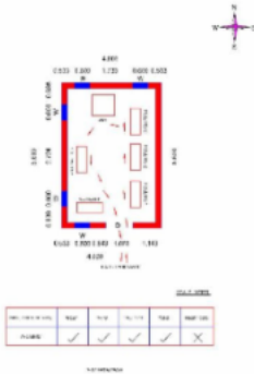
Cad View
