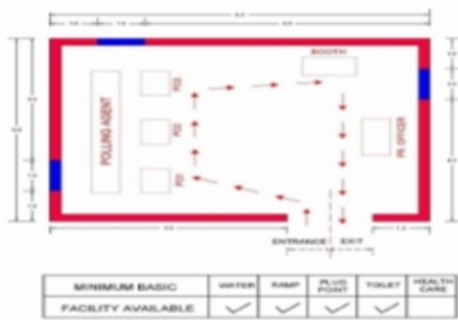
Cad View
