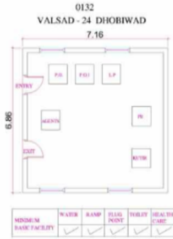
Cad View
