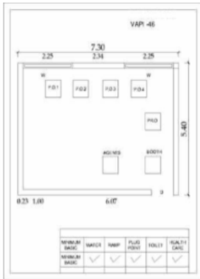
Cad View
