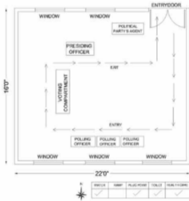
Cad View
