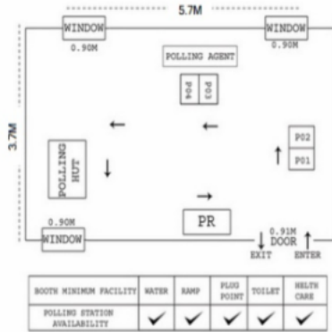
Cad View
