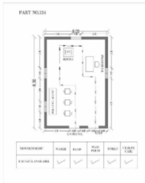
Cad View
