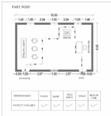
Cad View
