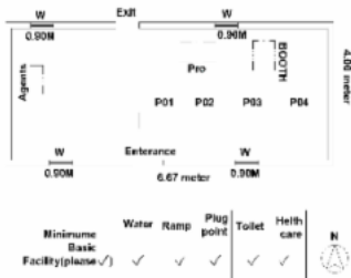
Cad Drowing of Polling Station Building Booth No-106 Katangtola
