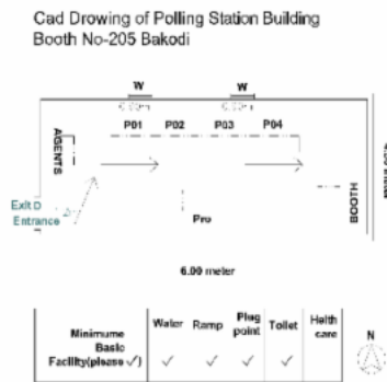
Cad View
