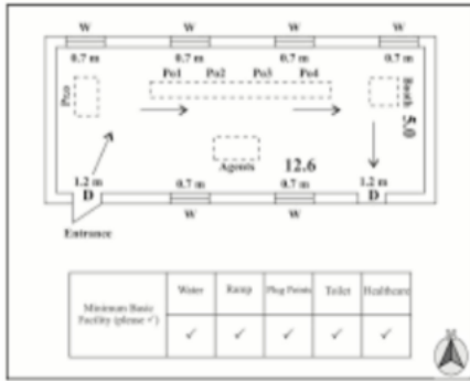
Sample CAD Drawing of Polling Station Building
