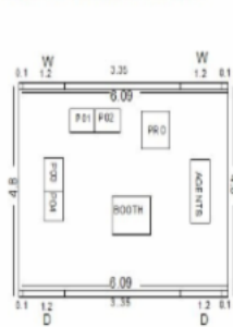
CAD LAYOUT OF POLLING BOOTH NO 91
