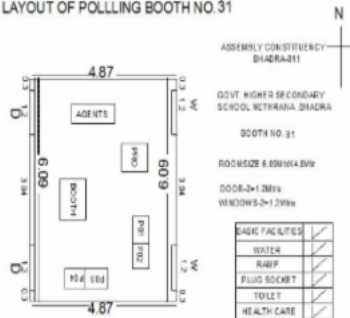
CAD LAYOUT OF POLLING BOOTH NO. 31
