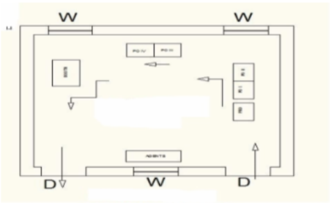
Cad View
