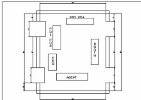
Cad View
