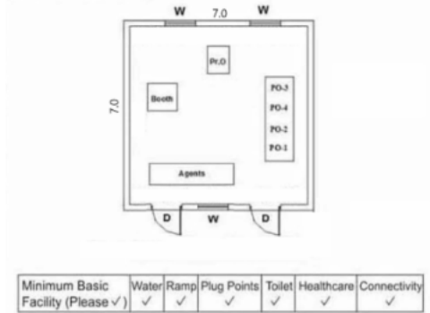
3. Cad Drawing
