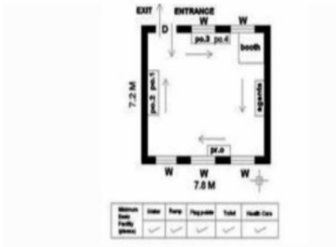
3. CAD Drawing
