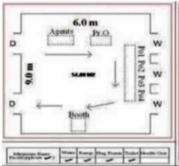
3. CAD Drawing
