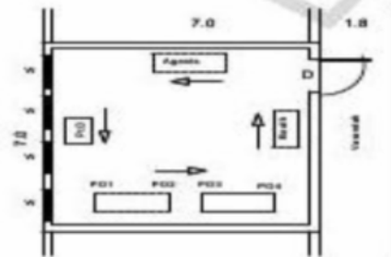
(3) CAD DRAWING
