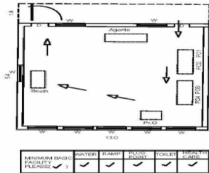
(3) CAD DRAWING
