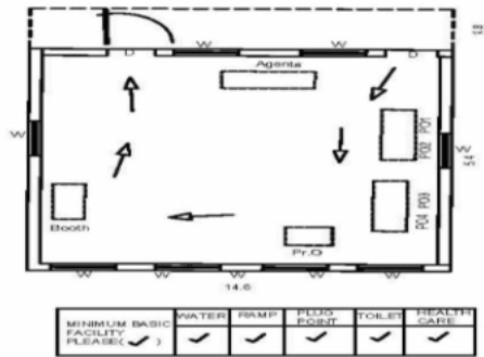
(3) CAD DRAWING
