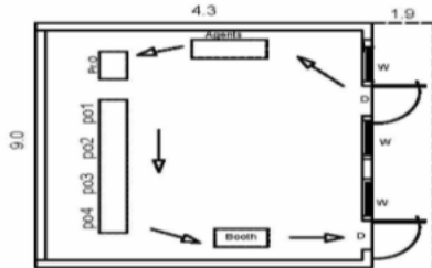
(3) CAD DRAWING
