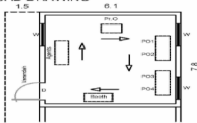
(3) CAD DRAWING
