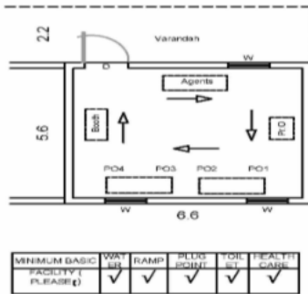
(3) CAD DRAWING
