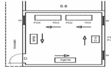
(3) CAD DRAWING
