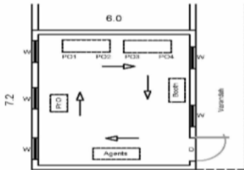
(3) CAD DRAWING
