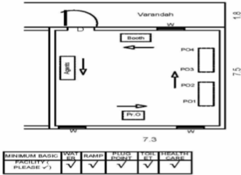
(3) CAD DRAWING
