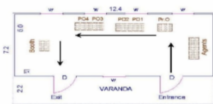
3.CAD Drawing
