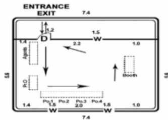
CAD DRAWING
