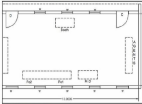
(3) CAD Drawing
