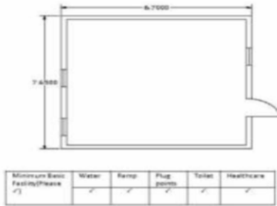
Cad Drawing
