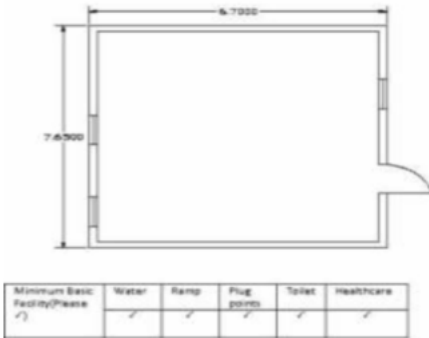
Cad Drawing
