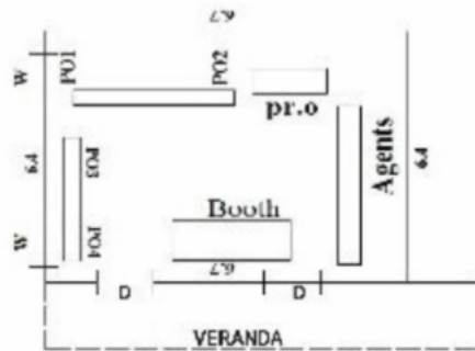
Cad Drawing
