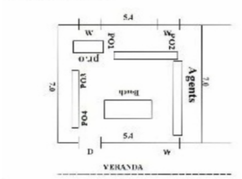
Cad Drawing
