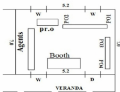
Cad Drawing
