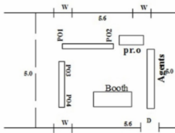
Cad Drawing
