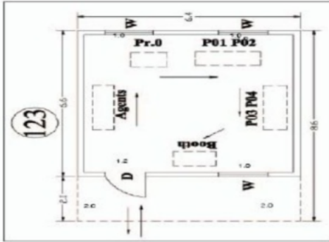
1) CAD Drawing
