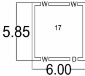
CAD DRAWING
