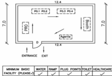
CAD Drawing.
