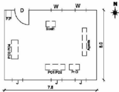
(3) CAD Drawing
